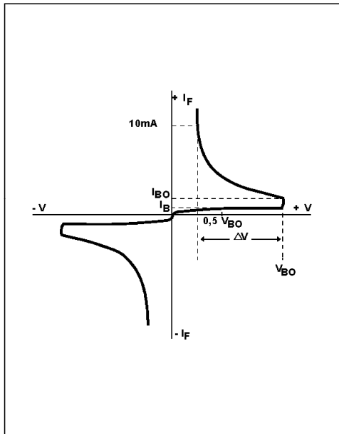
Diagram 1: Current-voltage characteristics
